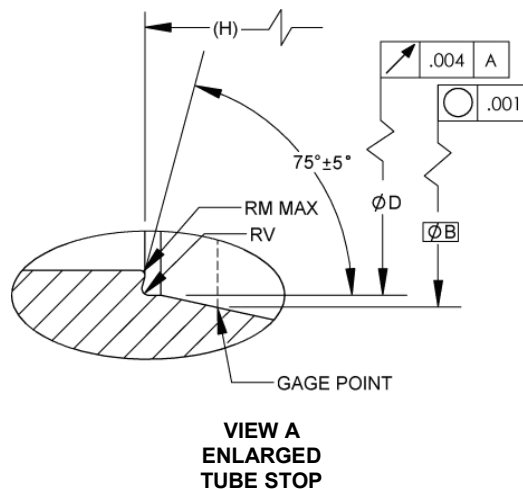
FIGURE 1 - FITTING END DESIGN, STYLE G
