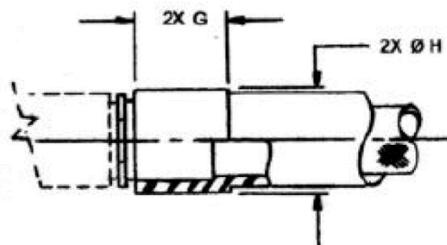
FIGURE 3 - INTEGRAL FIRESLEEVE CUFF – SEE TABLE 5 /13/
