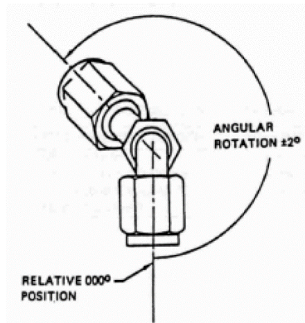
FIGURE 2 - FITTING ORIENTATION /17/
