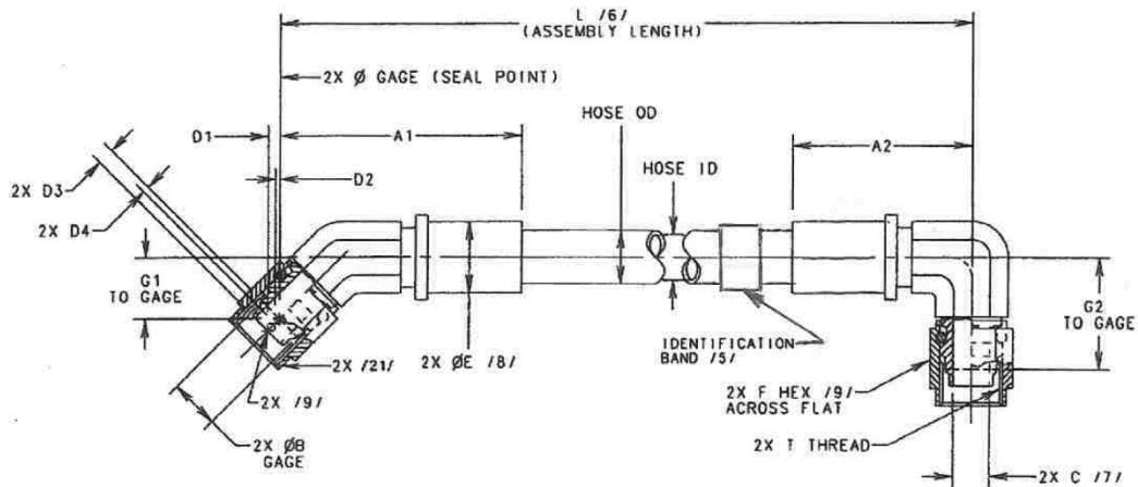
FIGURE 1 - HOSE ASSEMBLY DIMENSIONS – SEE TABLE 1
