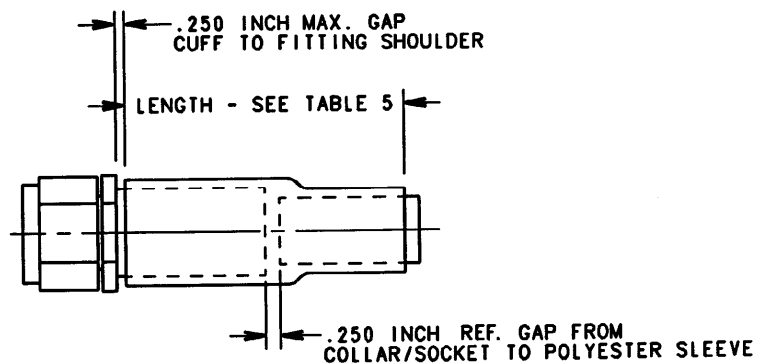
FIGURE 2 - POLYESTER ABRASION SLEEVE CUFF /20/
