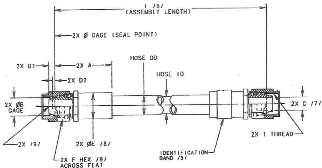
FIGURE 1 - FLARELESS HOSE ASSEMBLY, STRAIGHT TO STRAIGHT
