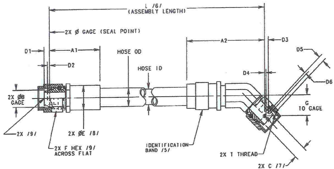
FIGURE 1 - FLARELESS HOSE ASSEMBLY, STRAIGHT TO 45 DEGREE ELBOW
