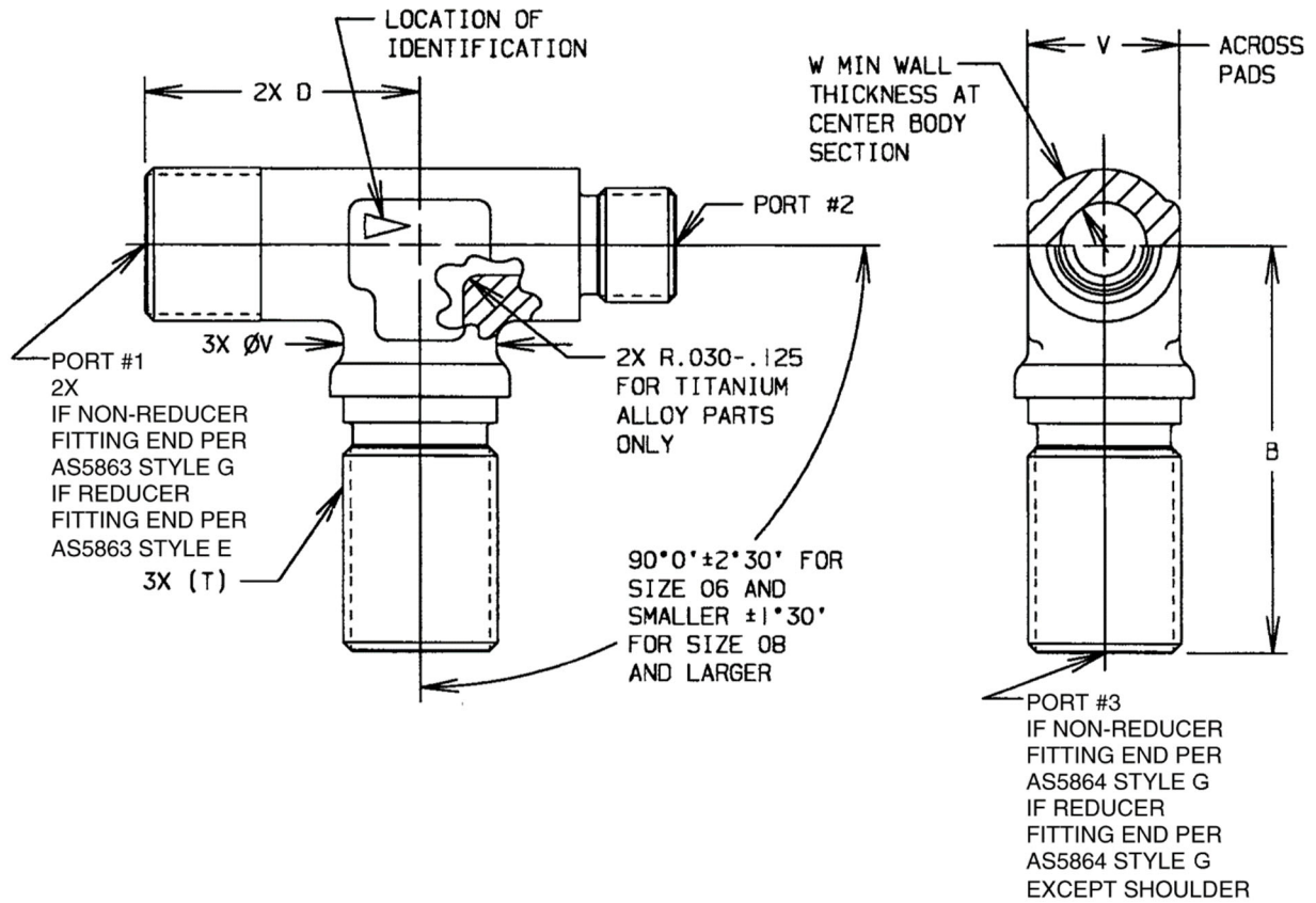
FIGURE 1 - FITTING, TEE, BULKHEAD END, PORT #2 SHOWN AS REDUCER
