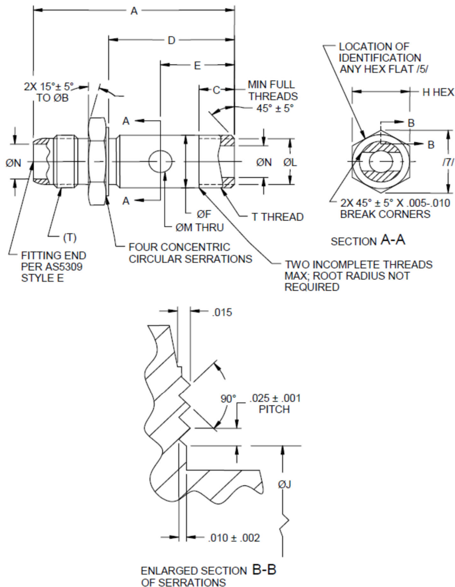
FIGURE 1 - FITTING, BOLT
