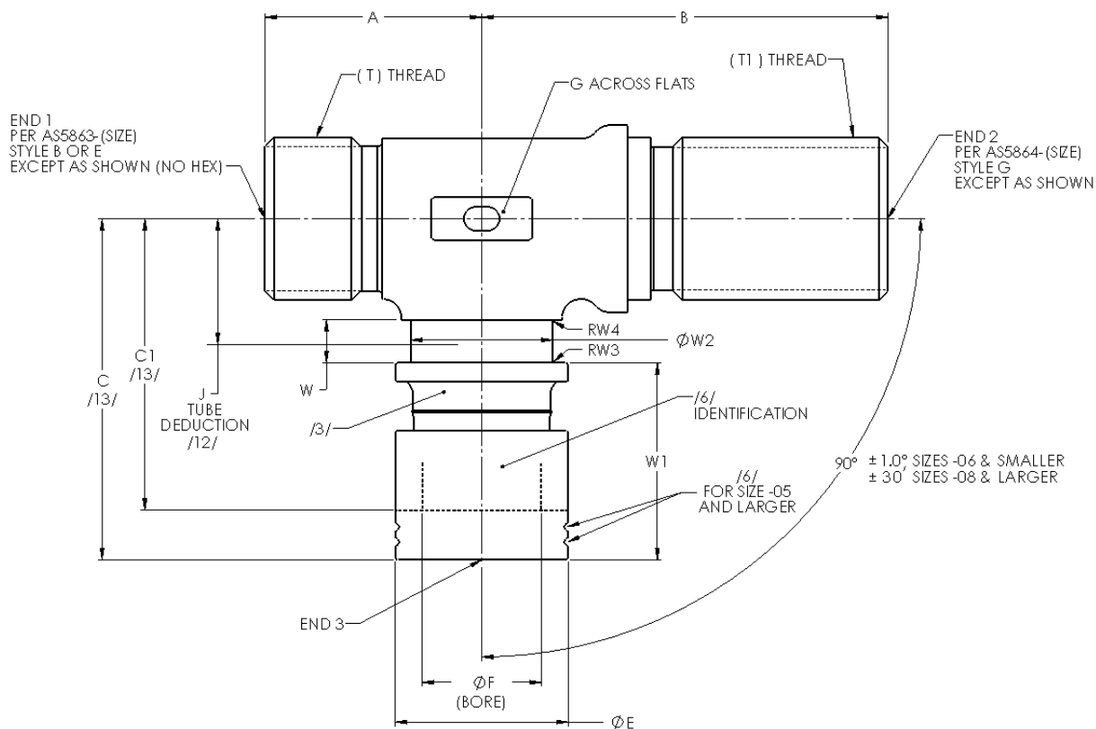
FIGURE 1 - TEE, MALE FLARELESS, BULKHEAD FLARELESS ON THE RUN, AXIALLY SWAGED ON THE SIDE
