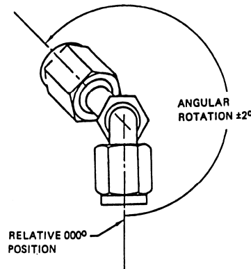
FIGURE 3 - FITTING ANGULAR ORIENTATION /19/
