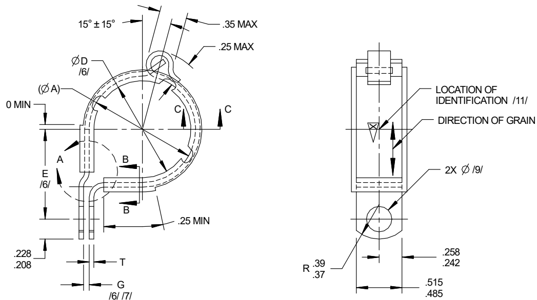
FIGURE 1 - CLAMP ASSEMBLY, LOOP
