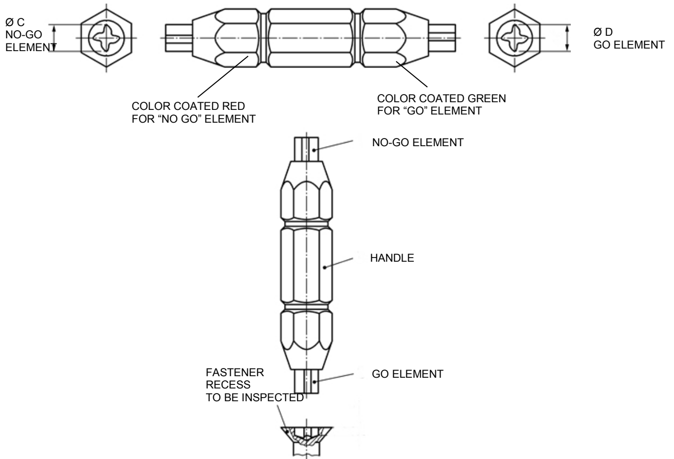
FIGURE 2 - GO/NO GO GAGE
