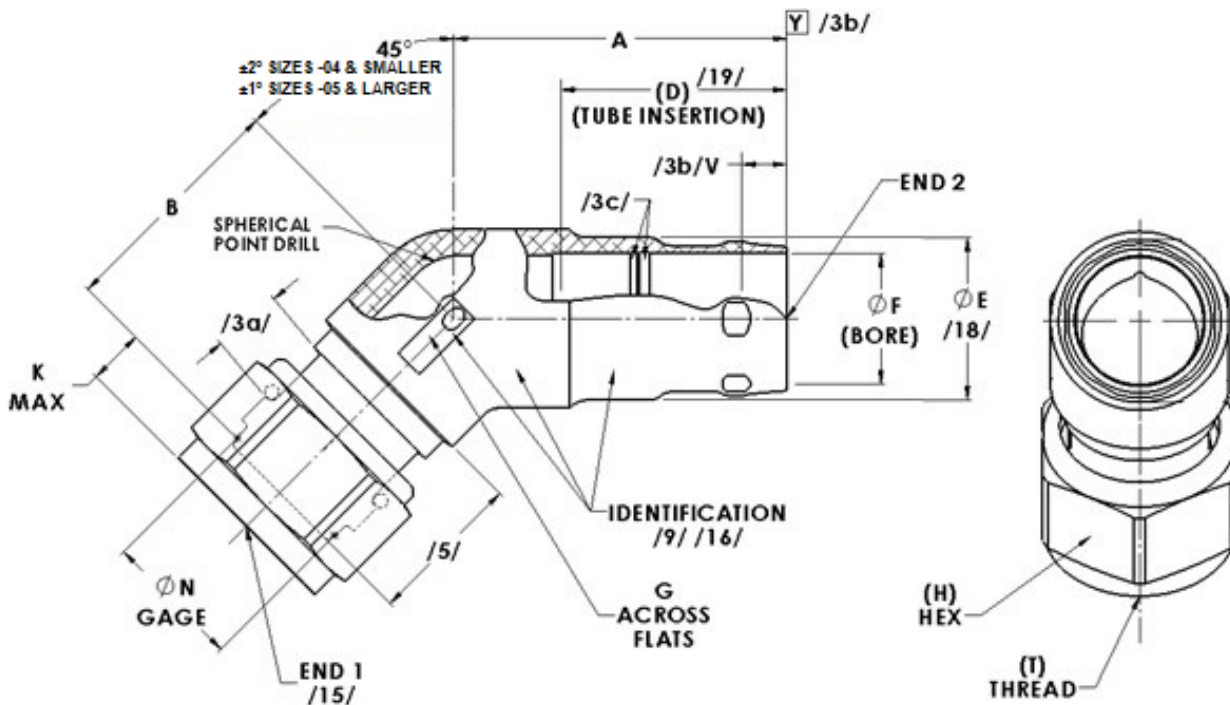
FIGURE 1 - ELBOW ASSEMBLY, SWIVEL ADAPTER, 45°, EXTERNAL SWAGE TO FLARELESS
