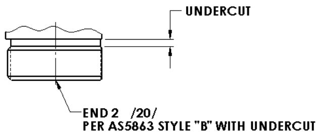
FIGURE 2 - FITTING END 2, SAME AS FIGURE 1 END 2, STYLE "B" SHOWN
