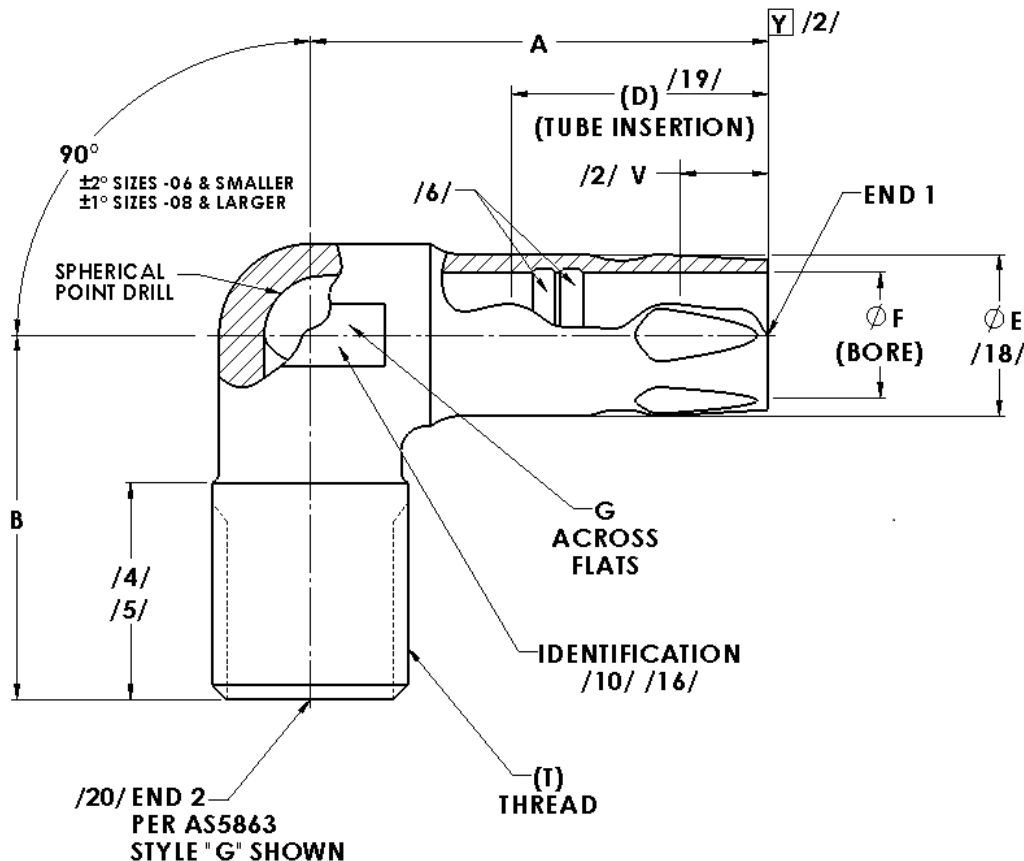
FIGURE 1 - ELBOW, 90°, EXTERNAL SWAGE TO FLARELESS
