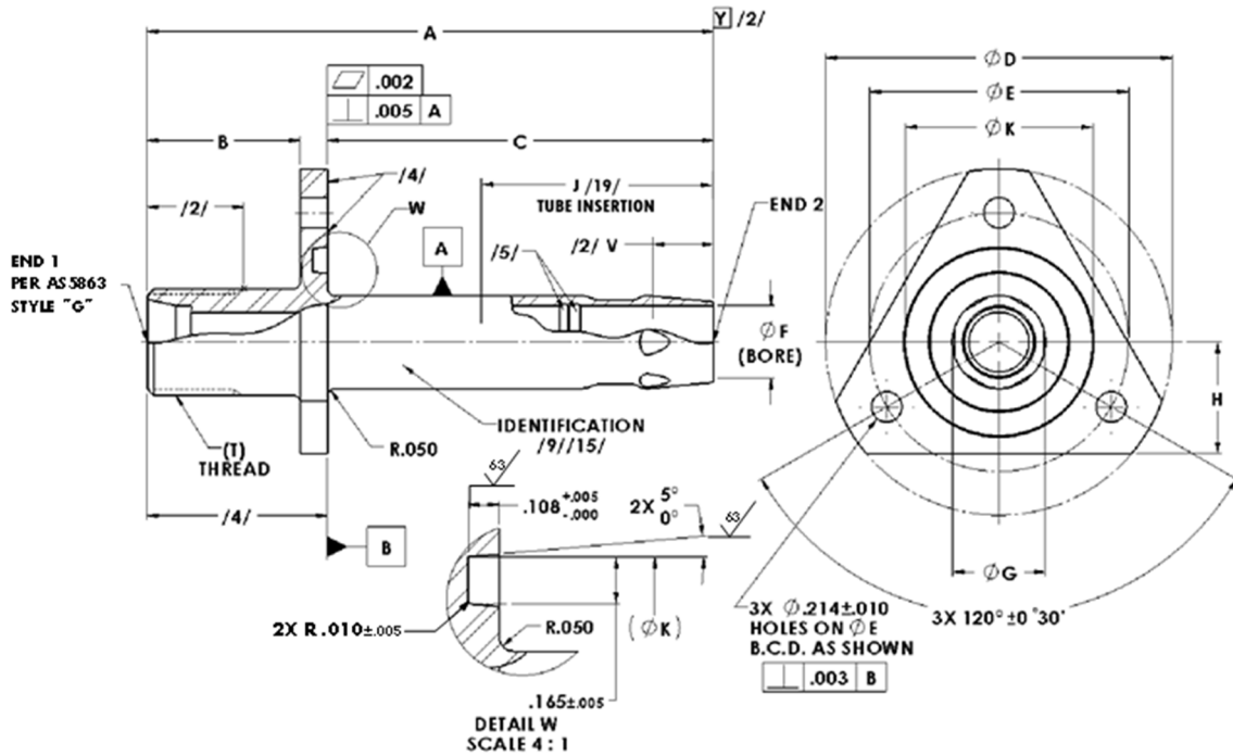
FIGURE 1 - ADAPTER, STRAIGHT, EXTERNAL SWAGE TO FLANGE SEALING, MALE FLARELESS
