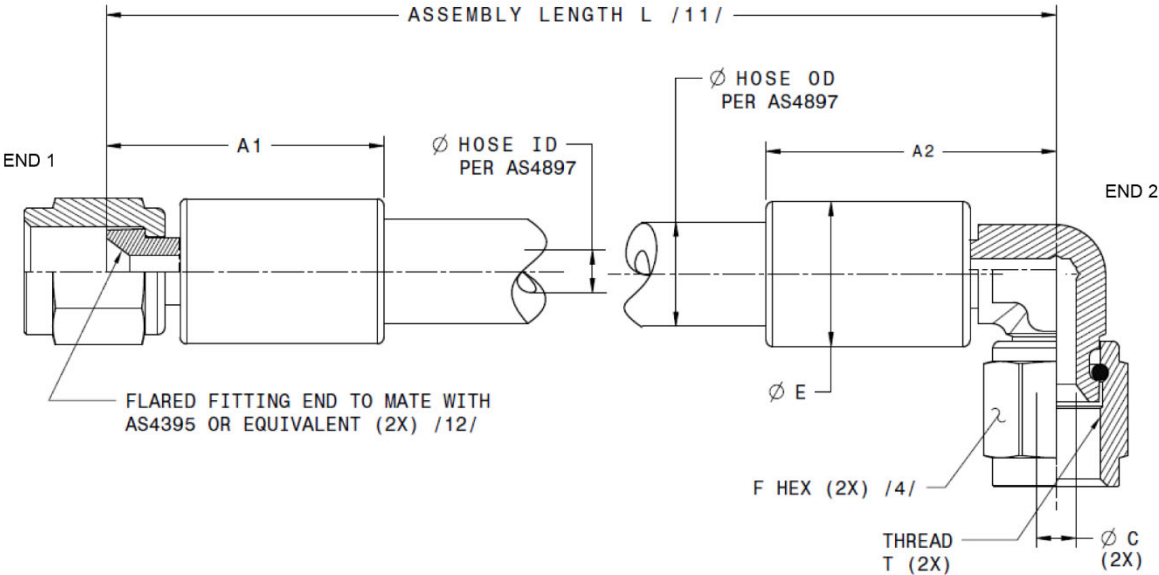
FIGURE 1 - HOSE ASSEMBLY
