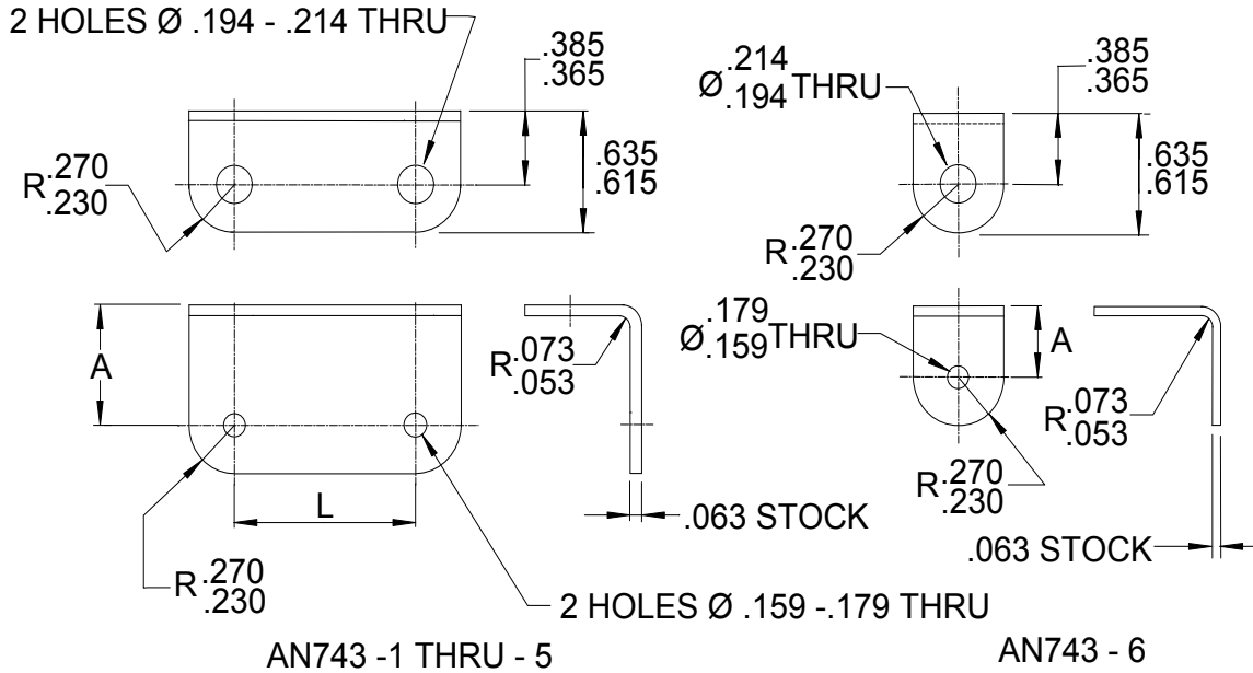
FIGURE 1 - BRACKETS
