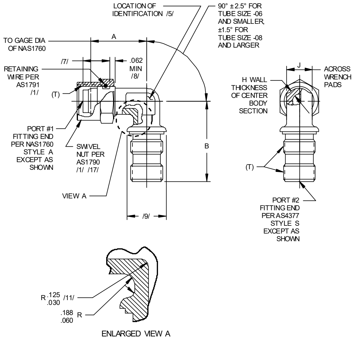
FIGURE 1 - FITTING ASSY, ELBOW, REDUCER, 90°, SWIVEL, BULKHEAD, REDUCED BODY, FLARELESS
