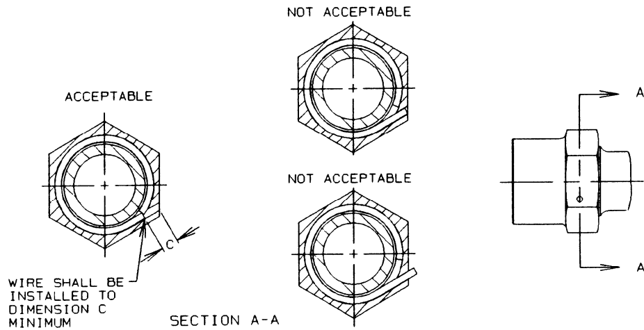
FIGURE 2 - INSTALLATION, SWIVEL NUT RETAINING WIRE
