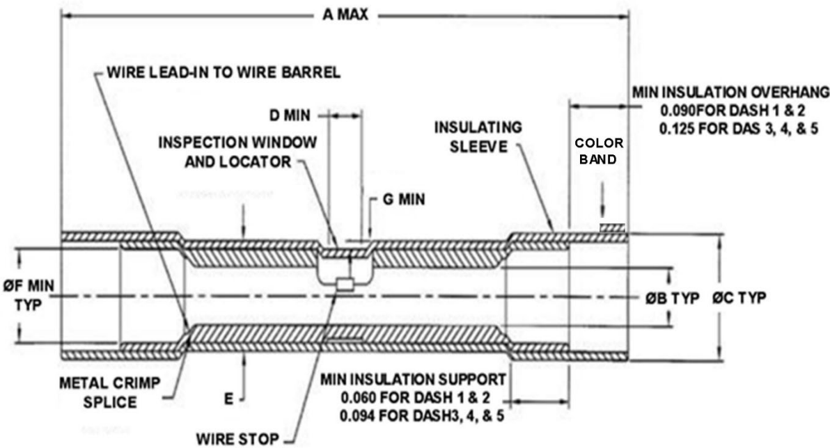
FIGURE 1 - SPLICE CONSTRUCTION
