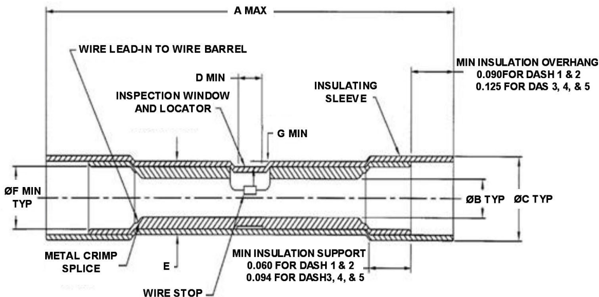
FIGURE 1 - SPLICE CONSTRUCTION
