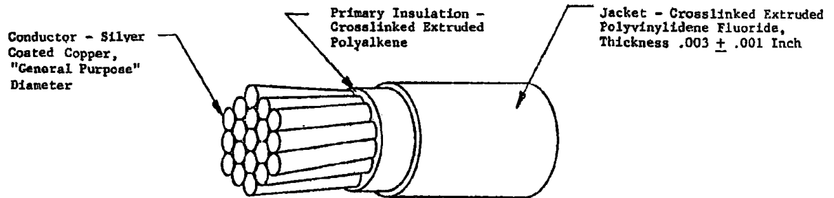
FIGURE 1 - AS81044/11 CONSTRUCTION
