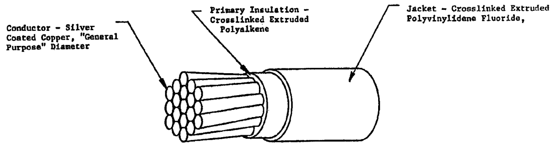
FIGURE 1 – AS81044/5 CONSTRUCTION
