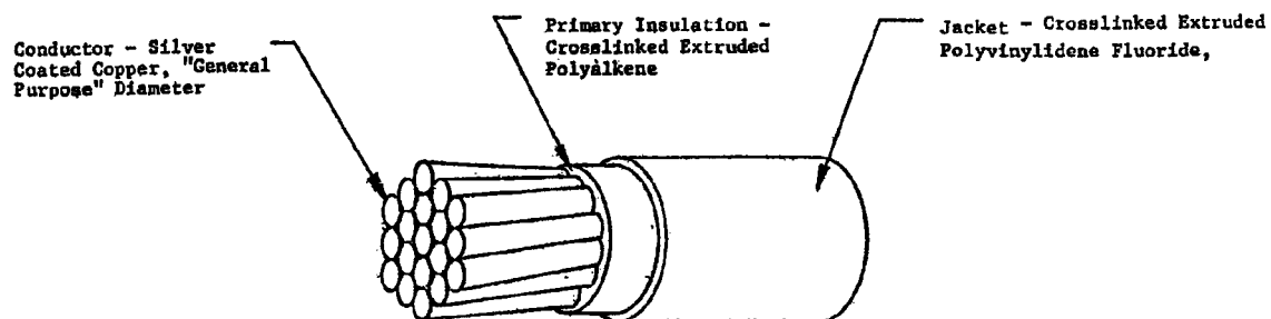
FIGURE 1 - AS81044/8 CONSTRUCTION
