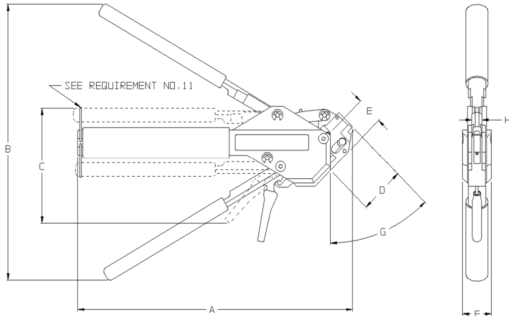
FIGURE 1 - DIMENSIONS AND CONFIGURATION (BAND INSTALLATION TOOL, SEE TABLE 1)
