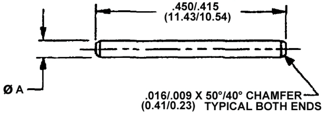
FIGURE 1 - SEALING CONTACT PLUG
