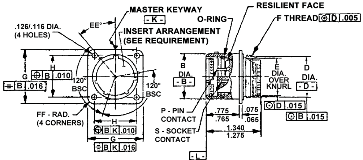
FIGURE 1 - CONNECTOR RECEPTACLE
