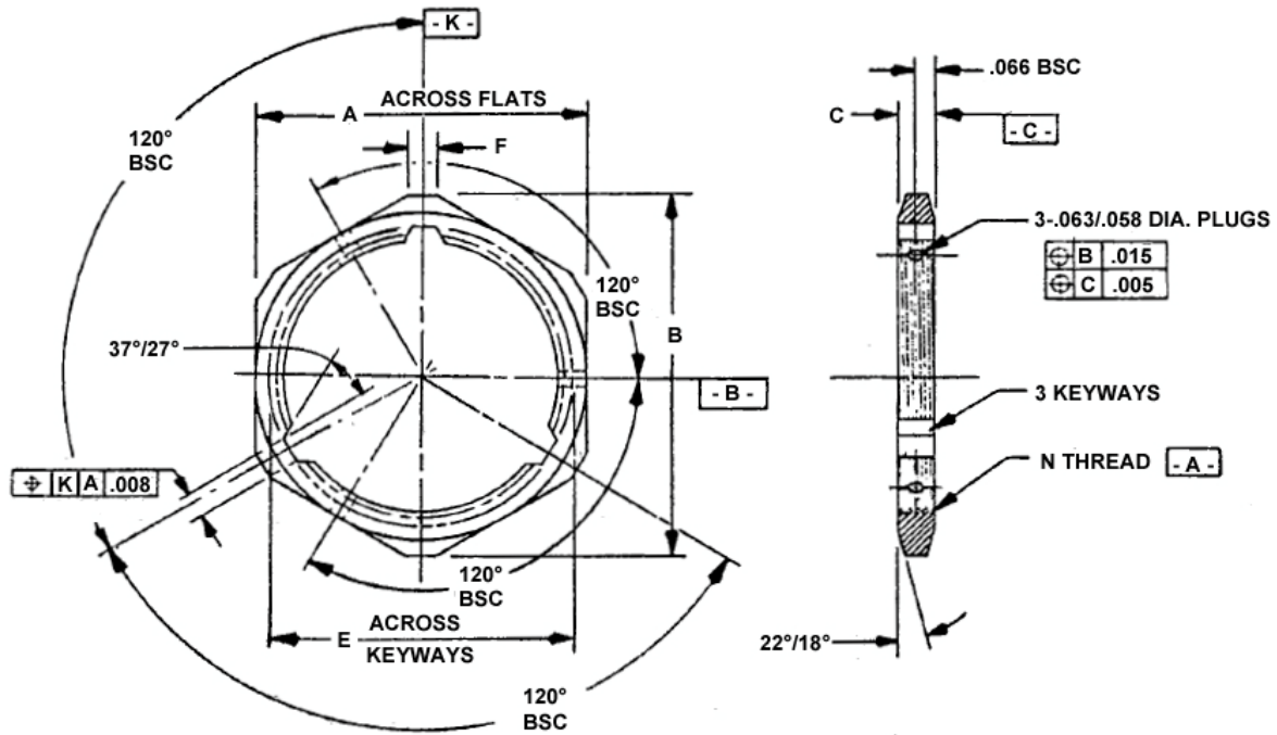
FIGURE 1 - CONNECTOR MOUNTING NUT
