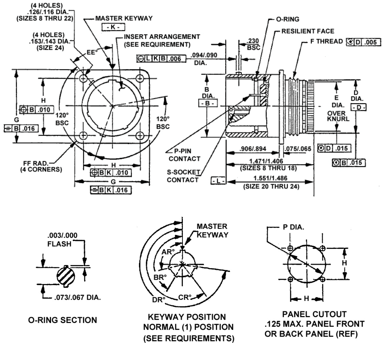
FIGURE 1 - CONNECTOR RECEPTACLE, FLANGE MOUNT
