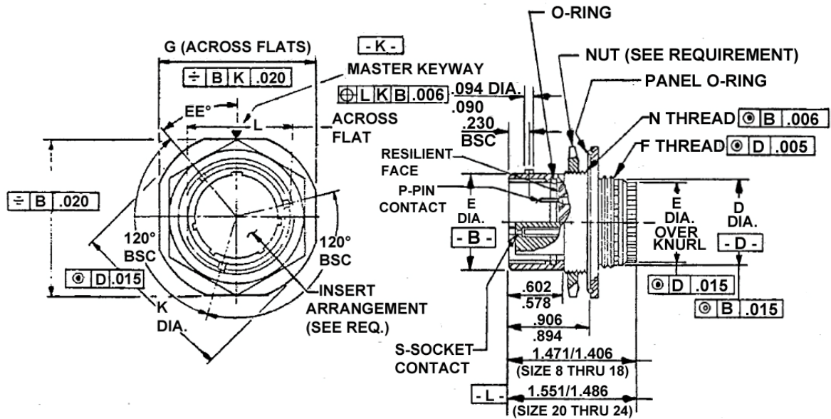
FIGURE 1 - CONNECTOR RECEPTACLE, JAM NUT MOUNT
