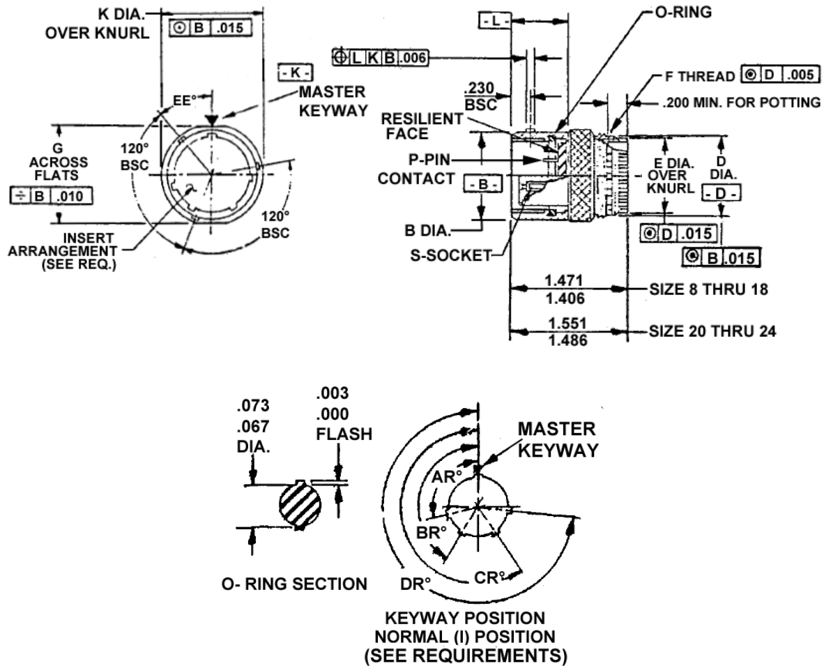
FIGURE 1 - CONNECTOR RECEPTACLE, CABLE CONNECTING
