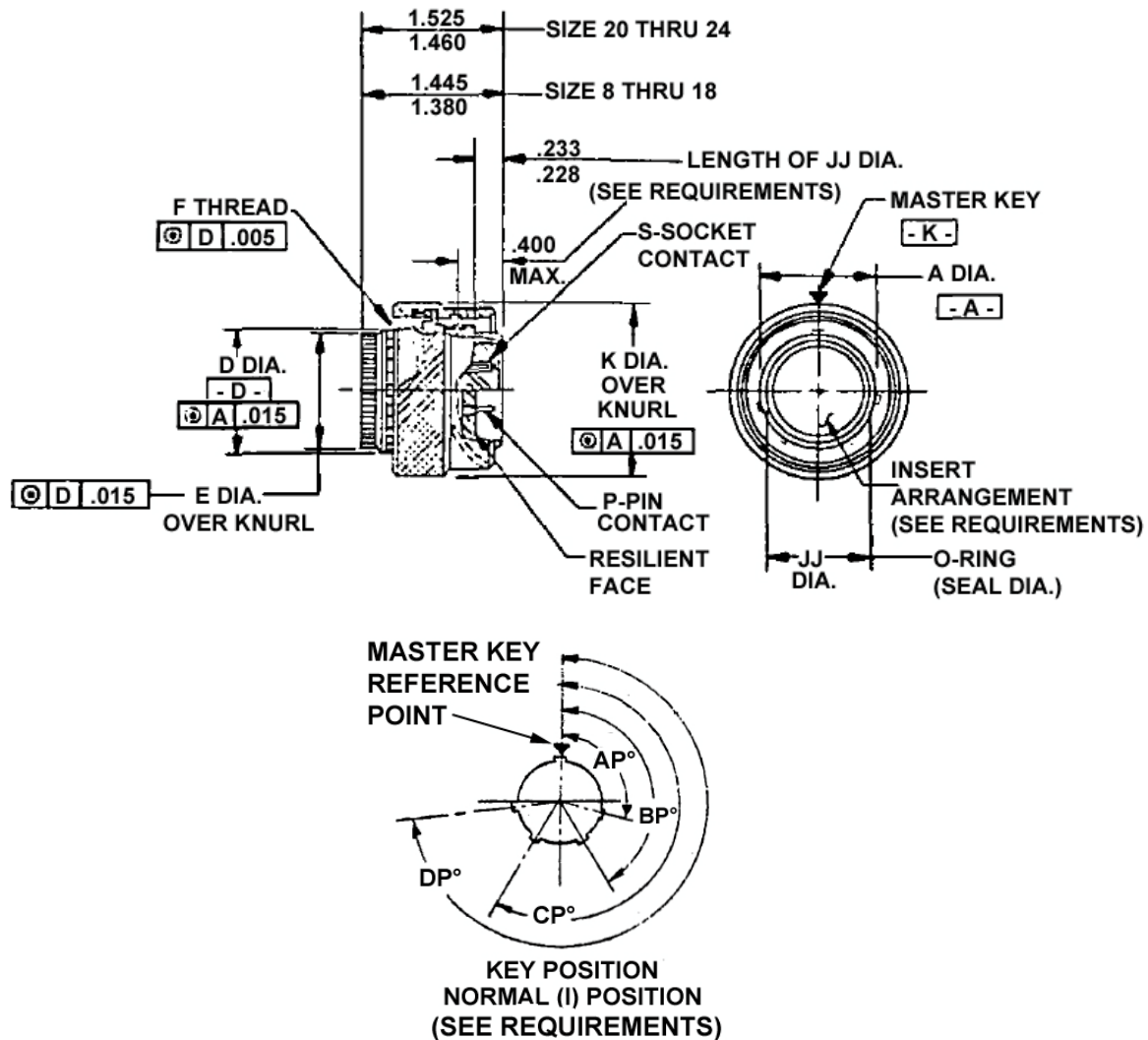
FIGURE 1 - CONNECTOR PLUG
