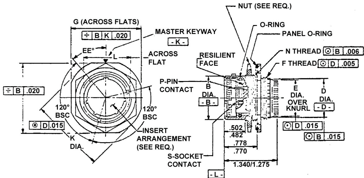
FIGURE 1 - CONNECTOR RECEPTACLE, JAM NUT MOUNT
