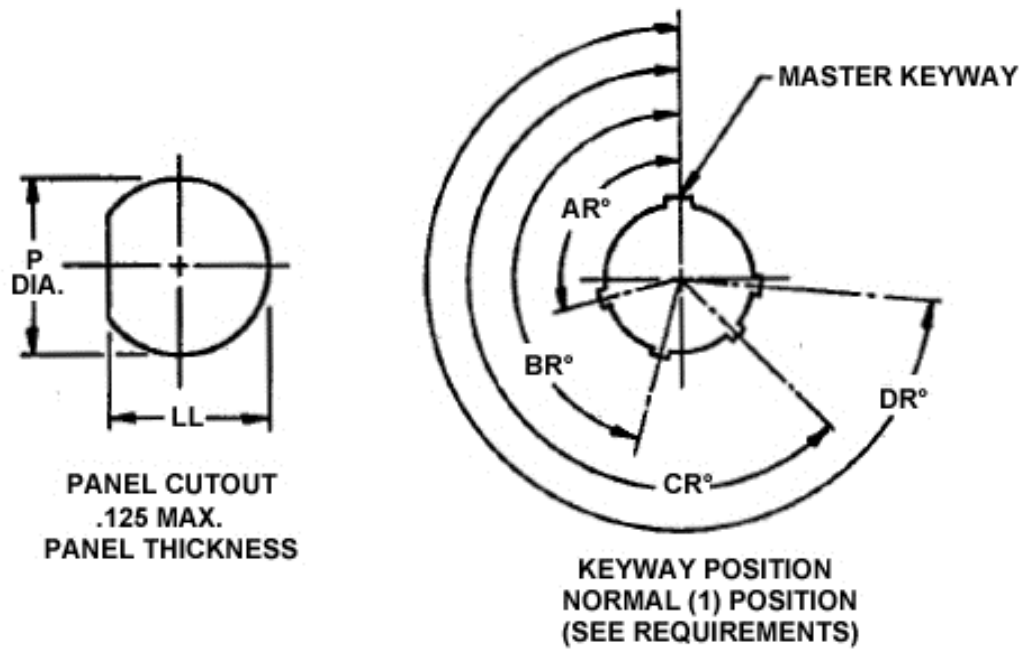
FIGURE 1 - CONNECTOR RECEPTACLE, JAM NUT MOUNT (SERIES 3) (CONTINUED)
