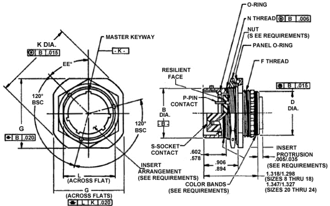
FIGURE 1 - CONNECTOR RECEPTACLE, JAM NUT MOUNT (SERIES 3)
