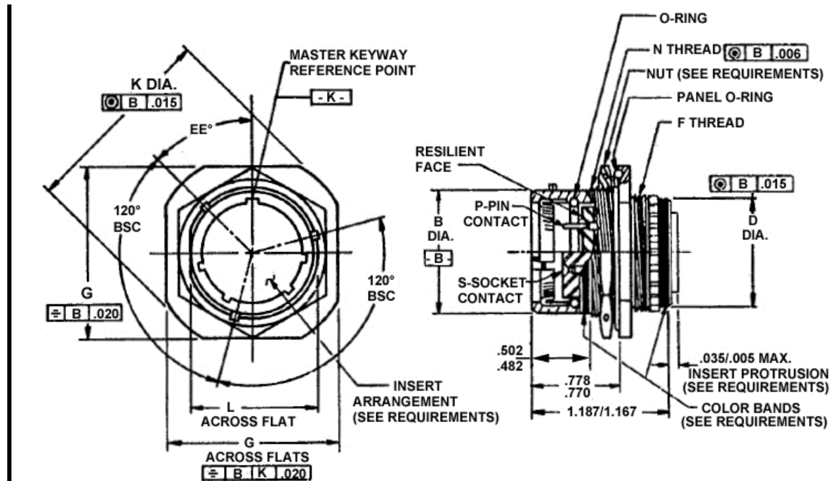
FIGURE 1 - CONNECTOR RECEPTACLE, JAM NUT MOUNT (SERIES 4)
