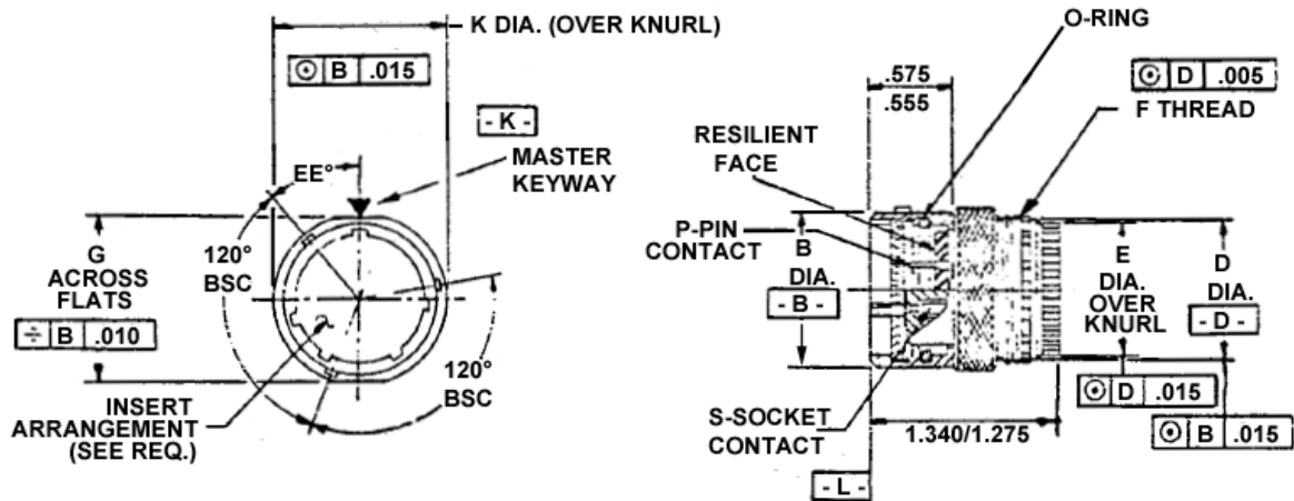
FIGURE 1 - CONNECTOR RECEPTACLE, CABLE CONNECTING
