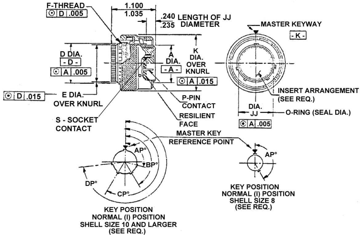
FIGURE 1 - CONNECTOR PLUG
