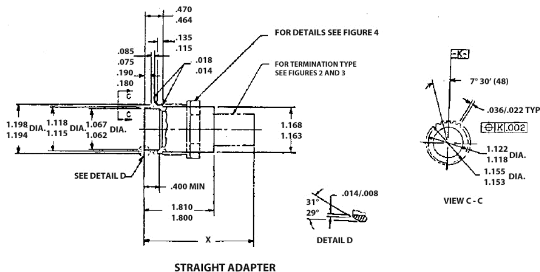
FIGURE 1 – ADAPTER CONFIGURATIONS
