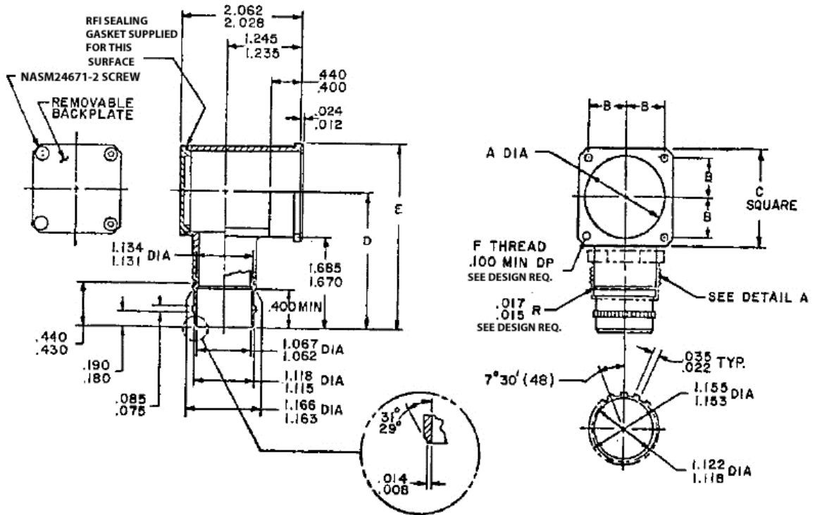
FIGURE 1 – CONNECTOR ADAPTER CONFIGURATION AND DIMENSIONS
