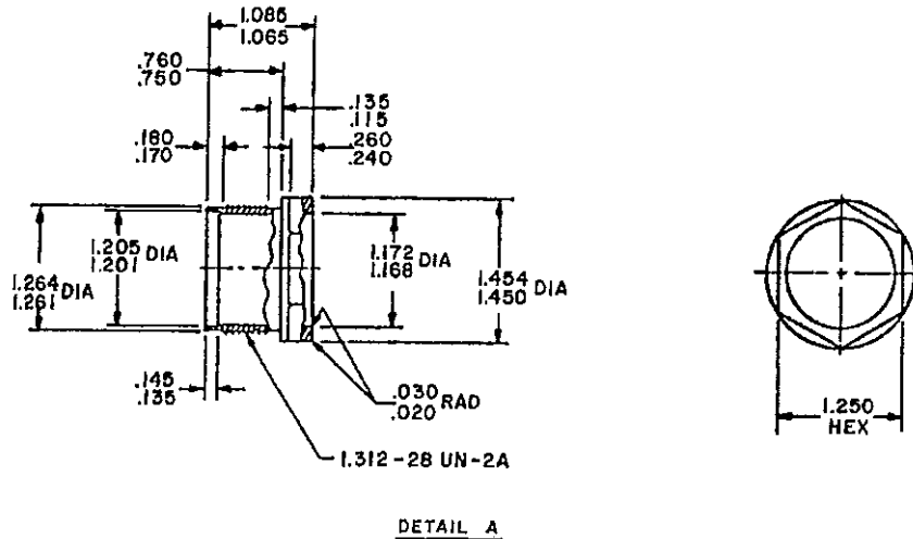
FIGURE 2 - CONNECTOR ADAPTER CONFIGURATION AND DIMENSIONS (DETAIL A)
