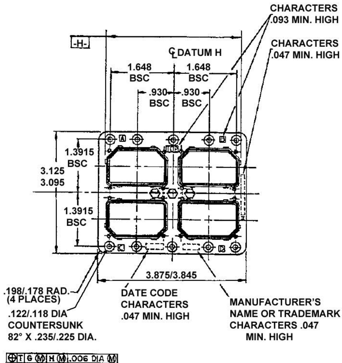
FIGURE 2 - CONNECTOR CONFIGURATIONS AND DIMENSIONS
