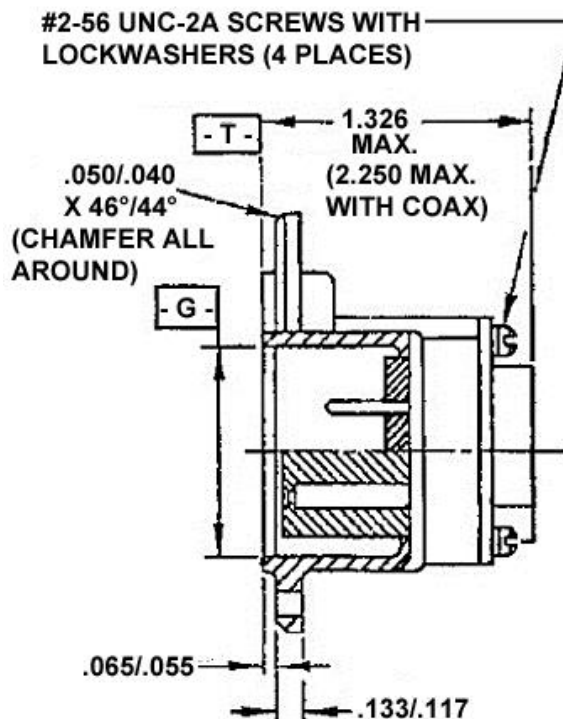
FIGURE 1 – CONNECTOR CONFIGURATION AND DIMENSIONS (CONTINUED)
