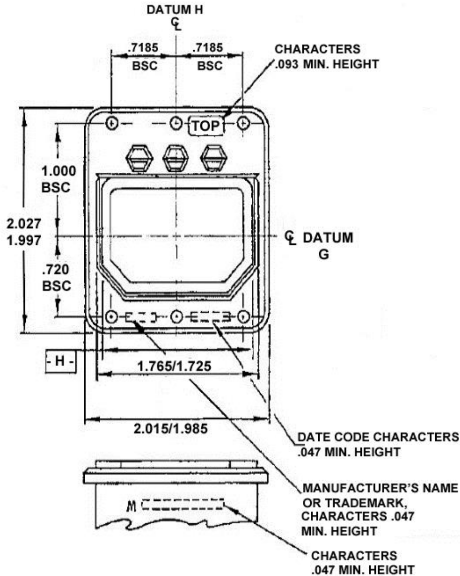
FIGURE 1 – CONNECTOR CONFIGURATION AND DIMENSIONS
