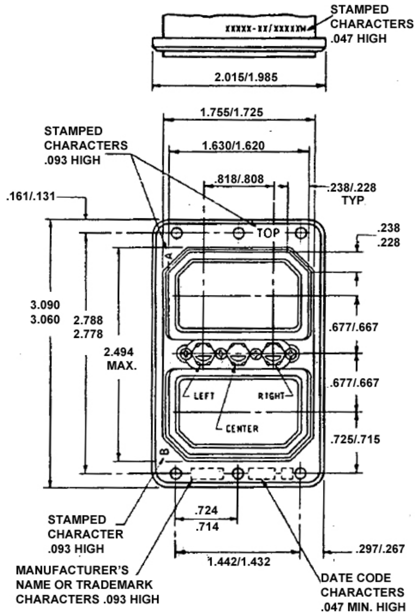
FIGURE 1 - CONNECTOR CONFIGURATIONS AND DIMENSIONS
