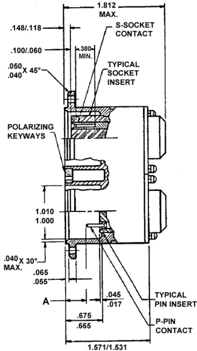
FIGURE 1 - CONNECTOR CONFIGURATIONS AND DIMENSIONS (CONTINUED)
