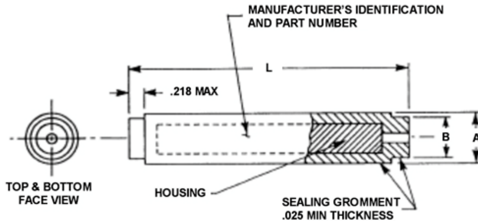
FIGURE 1 - WIRE IN-LINE JUNCTION SINGLE BODY - CONTACT SIZES 22, 20, 16, AND 12
