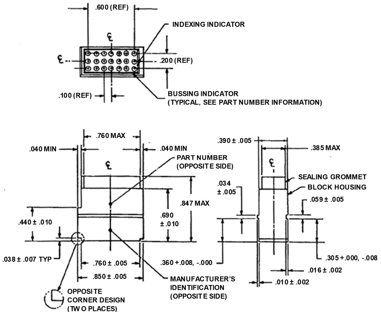
FIGURE 1 - TERMINAL JUNCTION BLOCK CONFIGURATION
