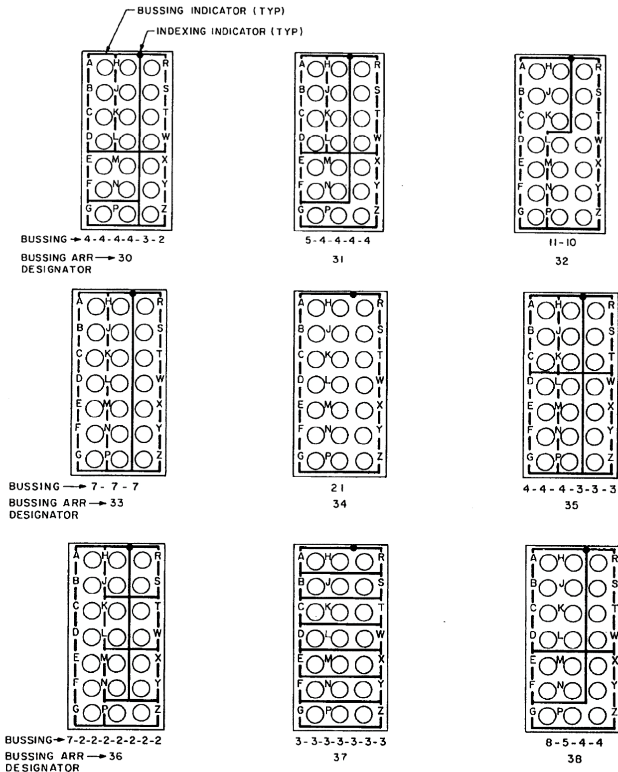
FIGURE 2 - AS81714/17 BUSSING ARRANGEMENTS (SEE FIGURE 1)
