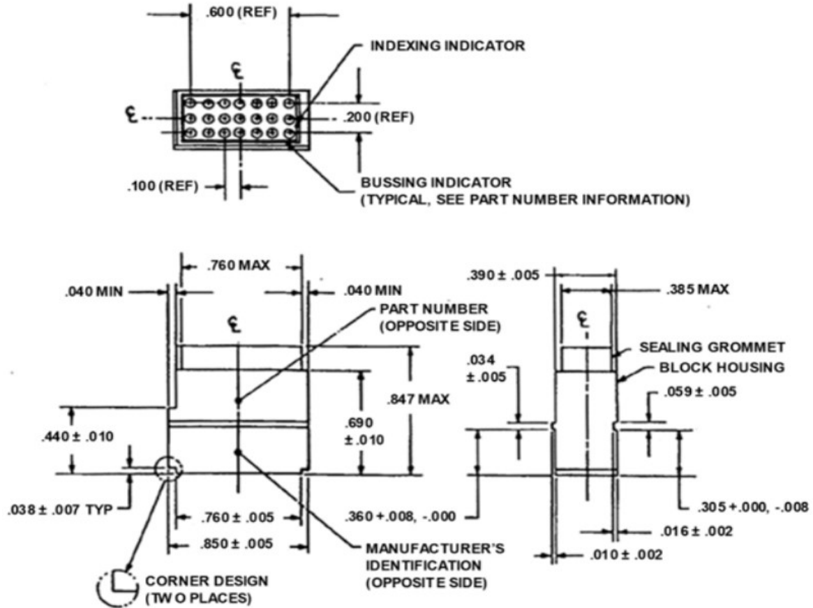
FIGURE 1 - TERMINAL JUNCTION BLOCK CONFIGURATION
