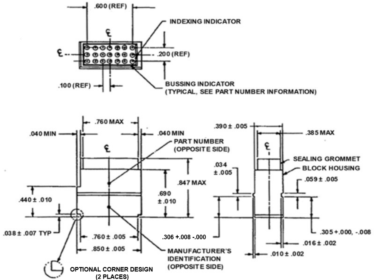
FIGURE 1 - TERMINAL JUNCTION BLOCK CONFIGURATION
