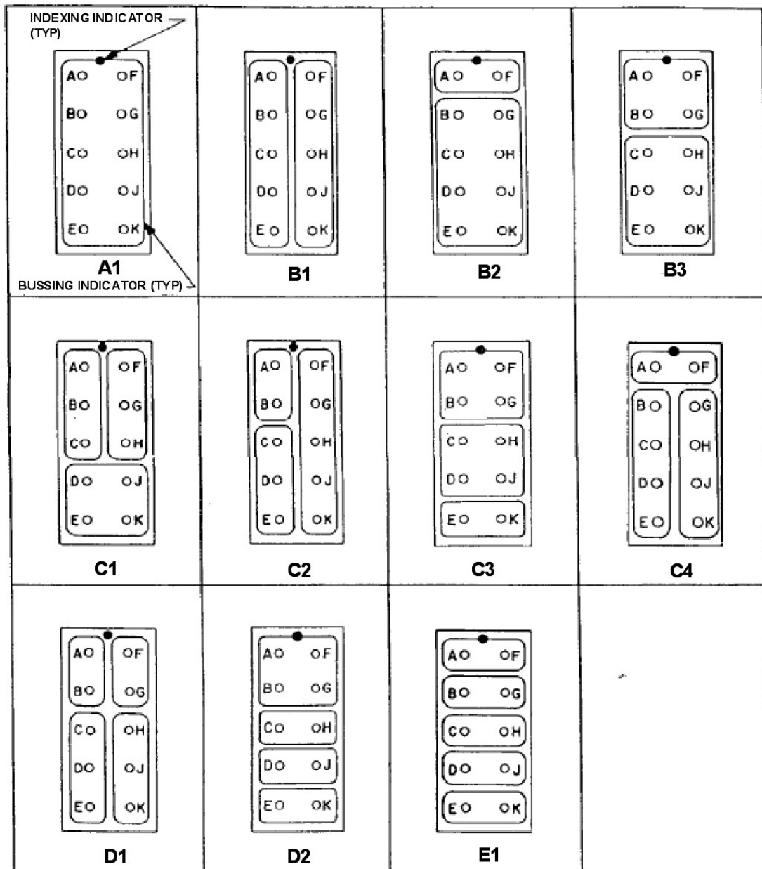
FIGURE 2 - AS81714/1 BUSSING ARRANGEMENTS (SEE FIGURE 1)
