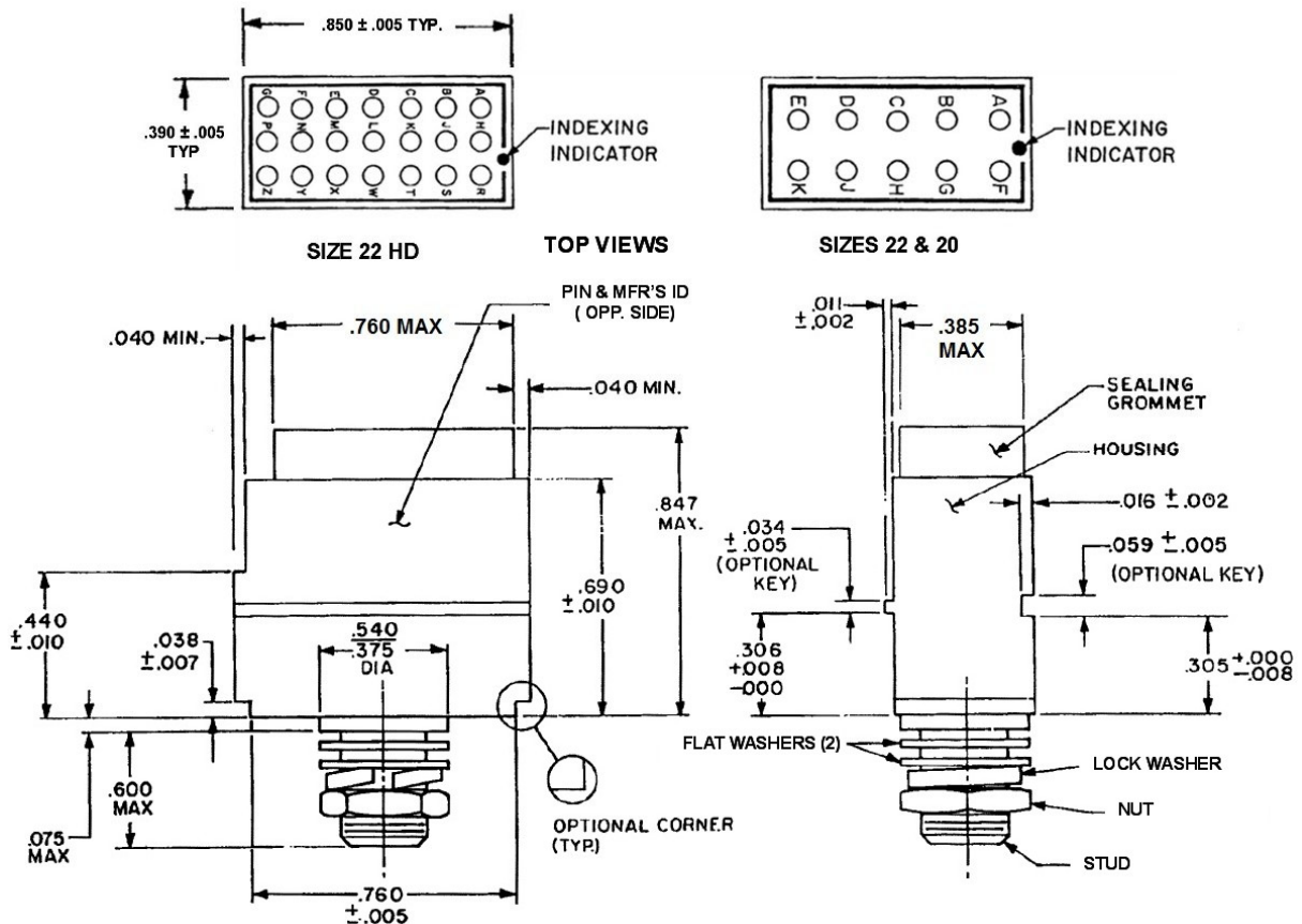
FIGURE 1 - GROUNDING BLOCKS, SIZES 22D, 22, AND 20
