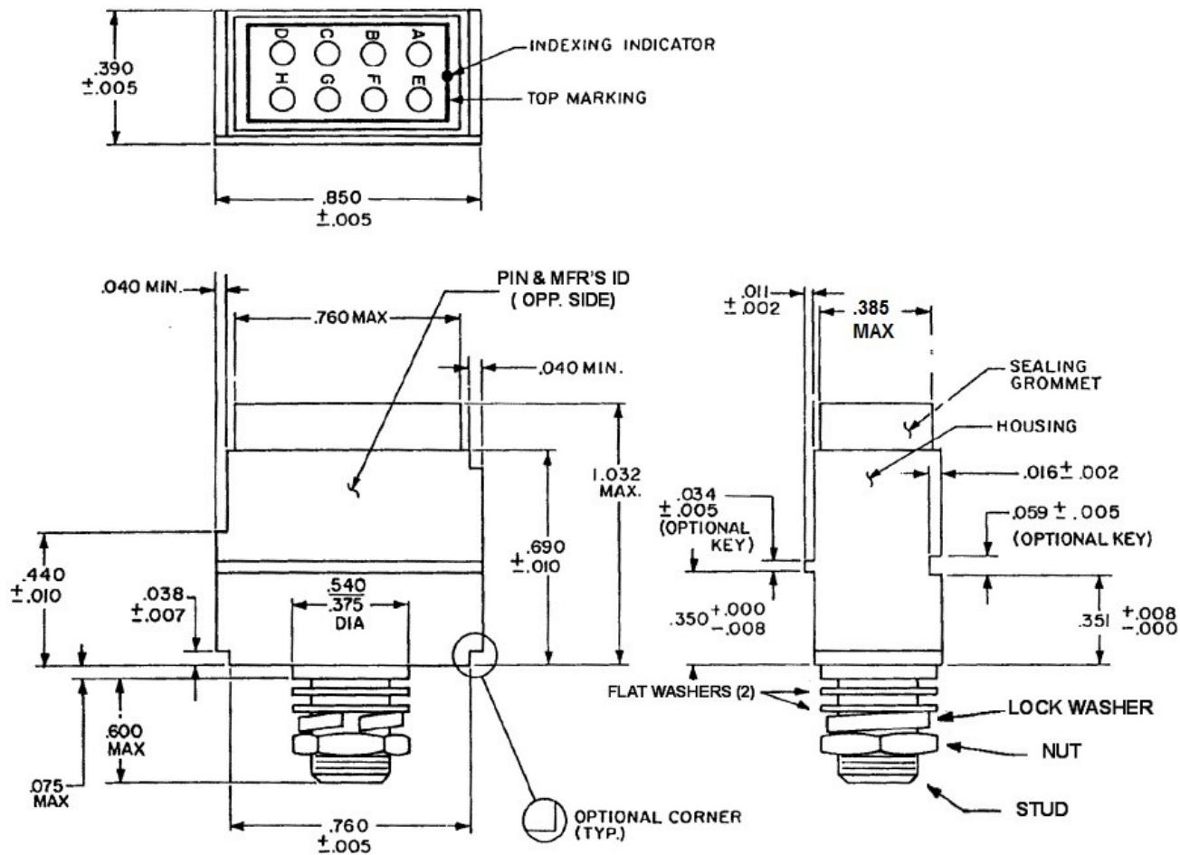
FIGURE 2 - GROUNDING BLOCK, SIZE 16
