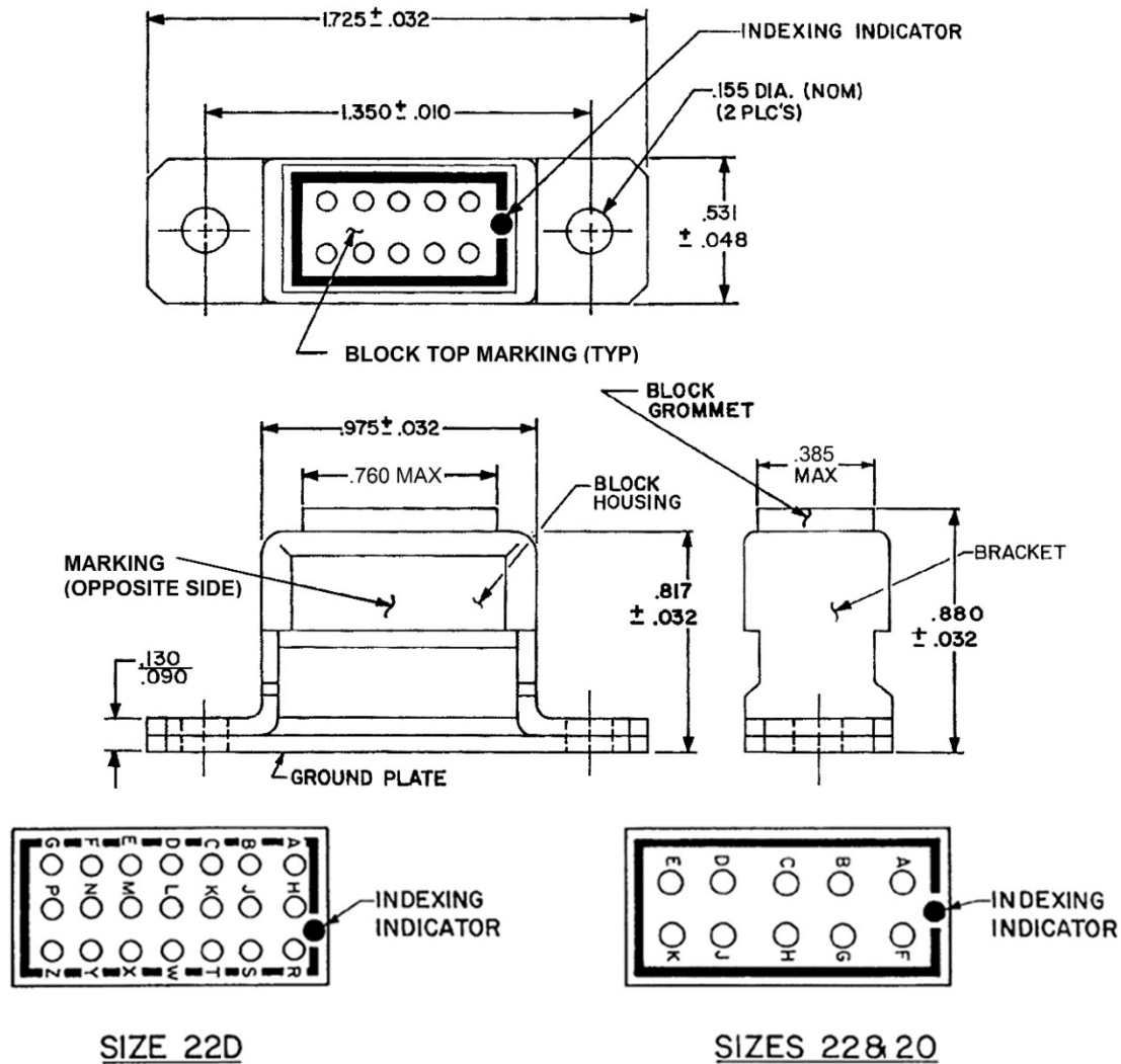
FIGURE 1 - MOUNTING BRACKET HOUSING ONE BLOCK: SIZE 22D, 22, AND 20
