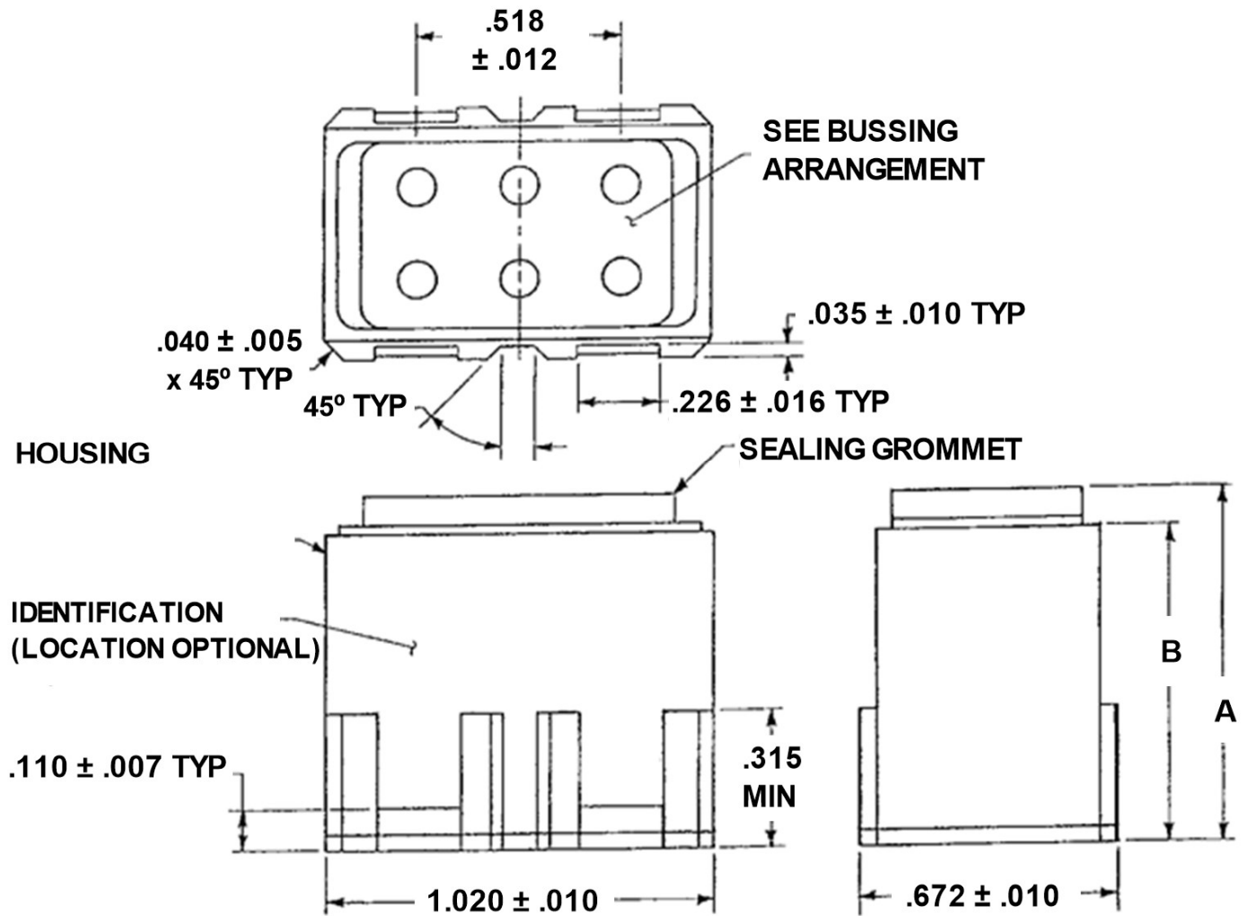
FIGURE 2 - COMPONENT MODULE (BLOCK) SIZE 12
