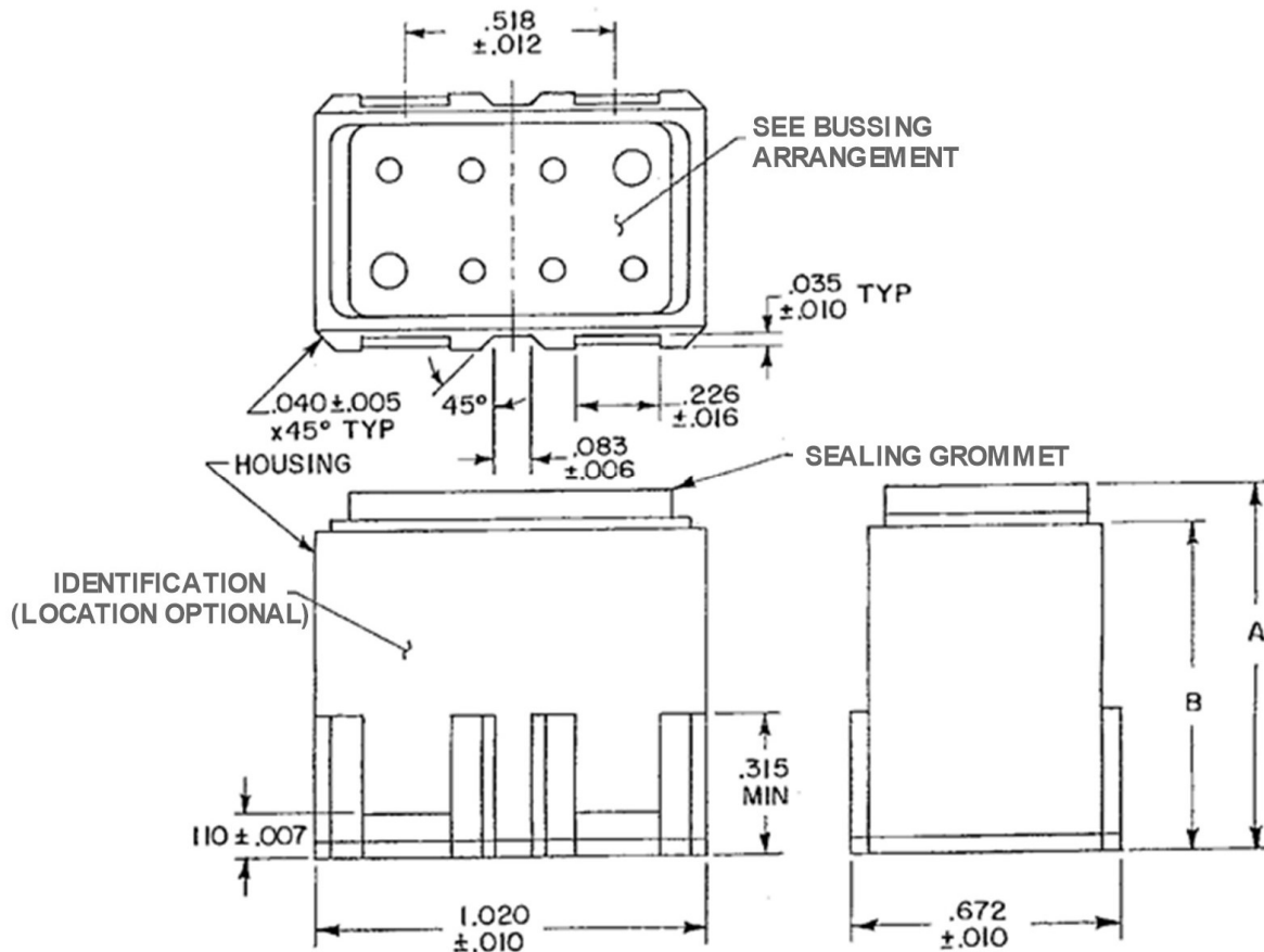
FIGURE 1 - COMPONENT (BLOCK) SIZE 0W, 0X, 0Z
