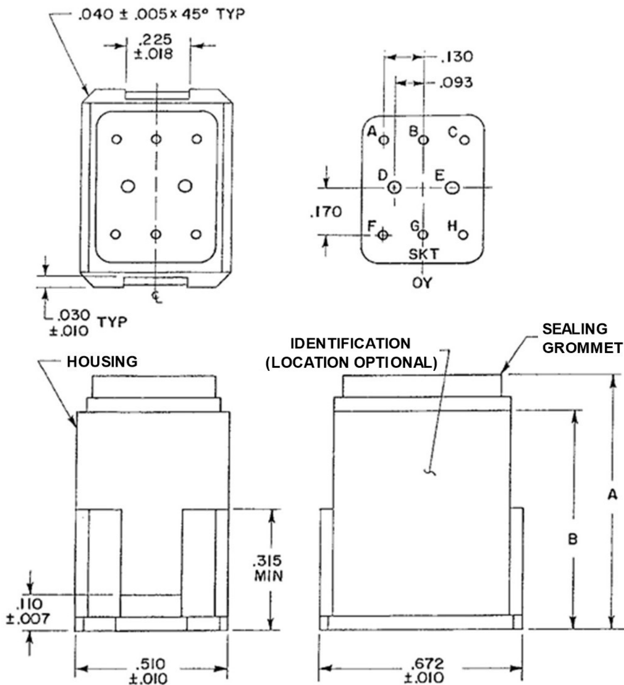
FIGURE 2 - COMPONENT (BLOCK) SIZE 0Y (CAVITIES D AND E SIZE 16 CONTACTS, A-C AND F-H SIZE 20 CONTACTS)
