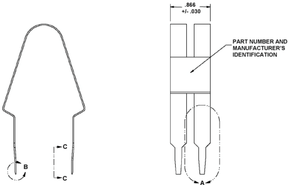
FIGURE 2 - BLOCK REMOVAL TOOL -2 TINE PAIRS SHOWN
