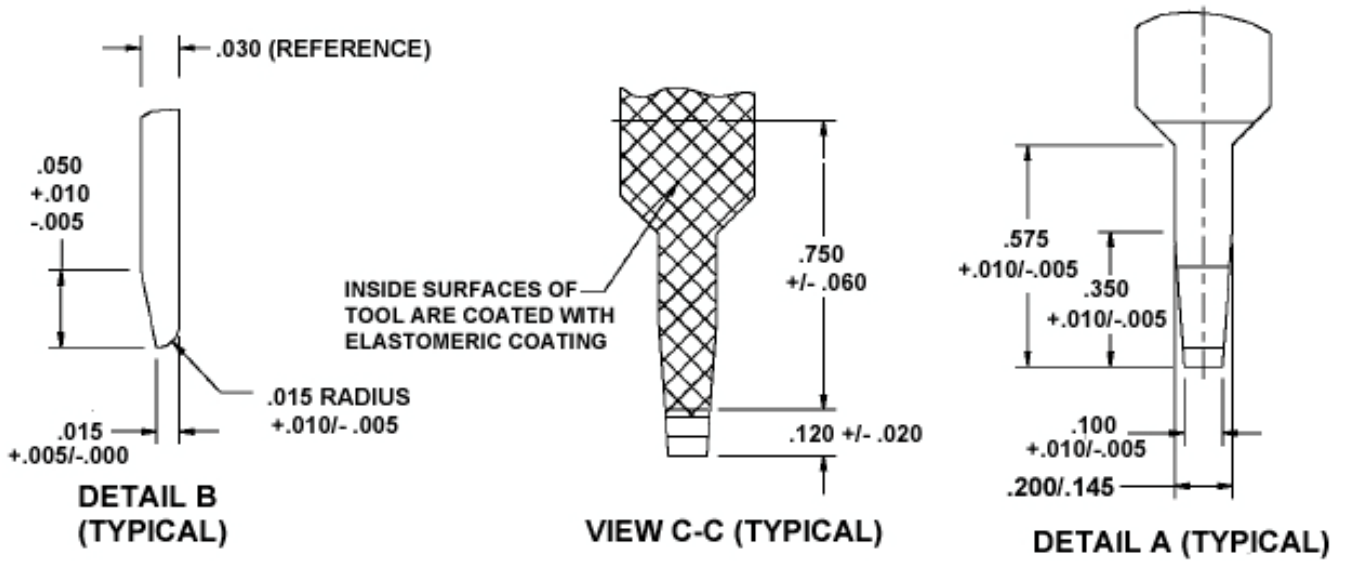
FIGURE 1 - BLOCK REMOVAL TOOL -1 TINE PAIR SHOWN (CONTINUED)
