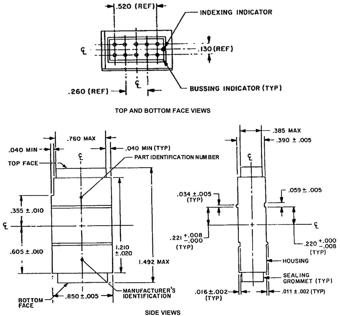
FIGURE 1 - FEED THRU TERMINAL JUNCTION BLOCK, SERIES 1 - CONTACT SIZE 22
